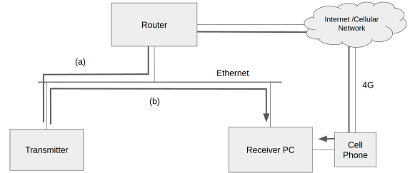
Figure 4. NETWORK CONFIGURATION.
